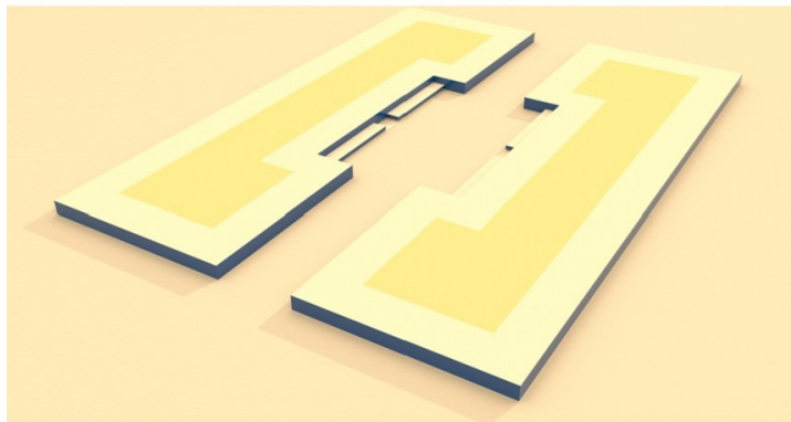
Tol-e Ajori. 3D graphic reconstruction. Dark yellow: mud-brick core; light yellow: baked bricks sections; blue: glazed bricks facing (Elaboration: S. Tilia)
